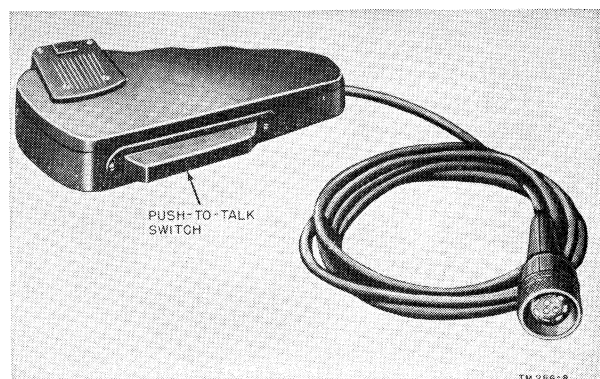
Figure 15. Microphone M-29/U.
